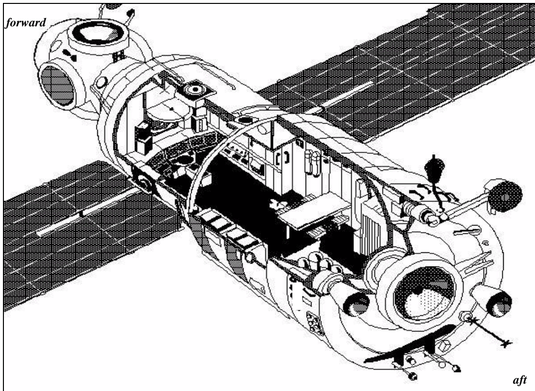
The Service Module is derived from and similar in design to the Mir Space Station Core Module.
